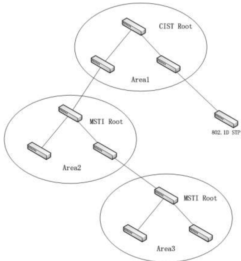
Figure 2.1 MSTP topology
